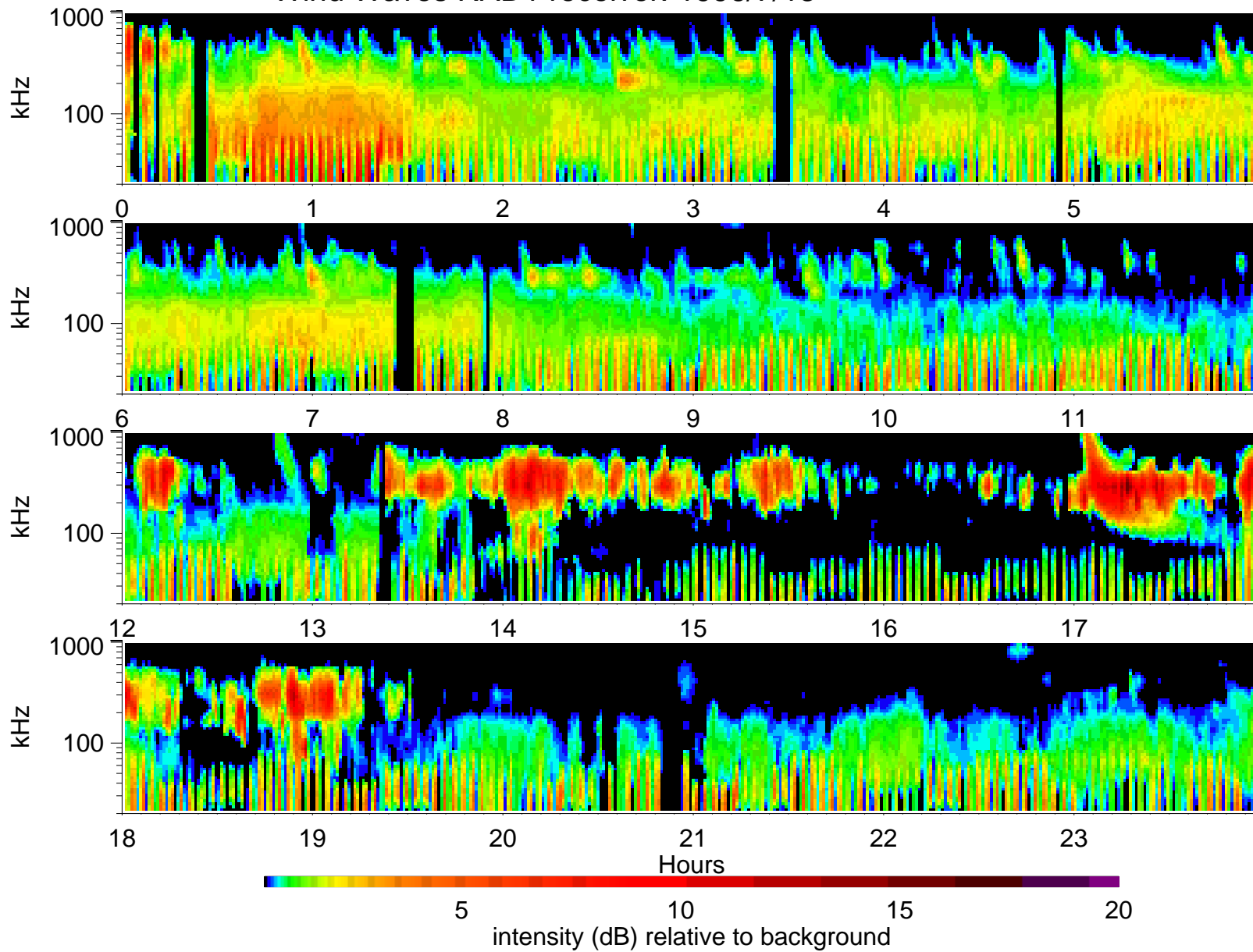
Wind Waves RAD1 receiver: 1996/7/13
