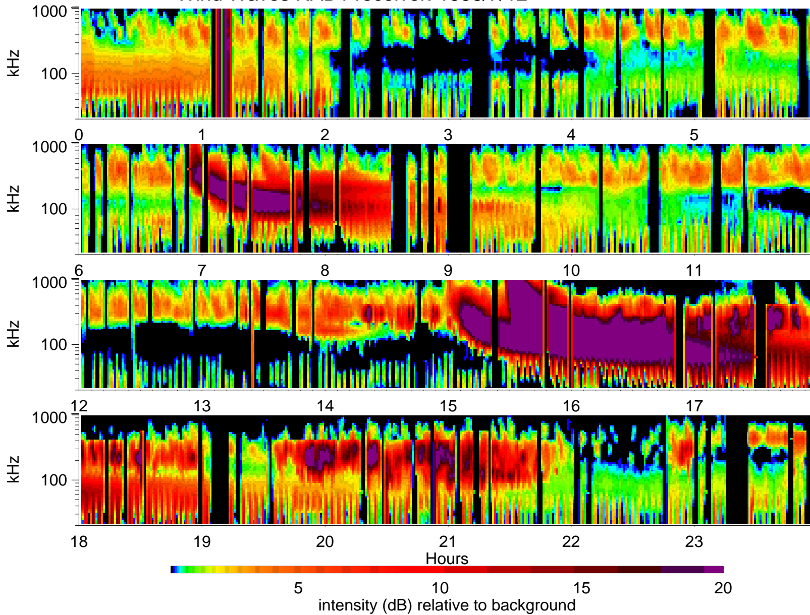
Wind Waves RAD1 receiver: 1996/7/12
