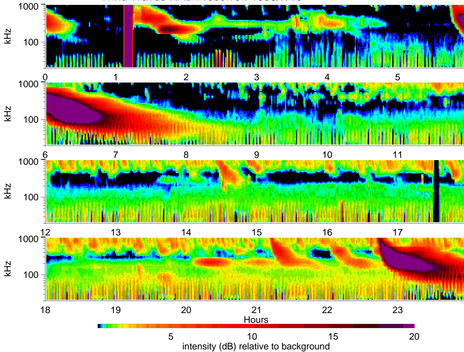
Wind Waves RAD1 receiver: 1996/7/10
