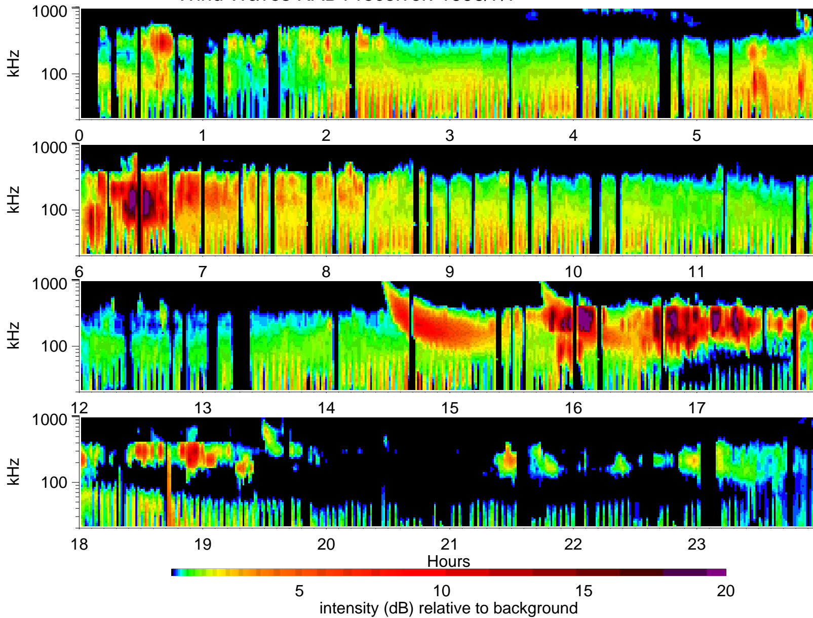
Wind Waves RAD1 receiver: 1996/7/7
