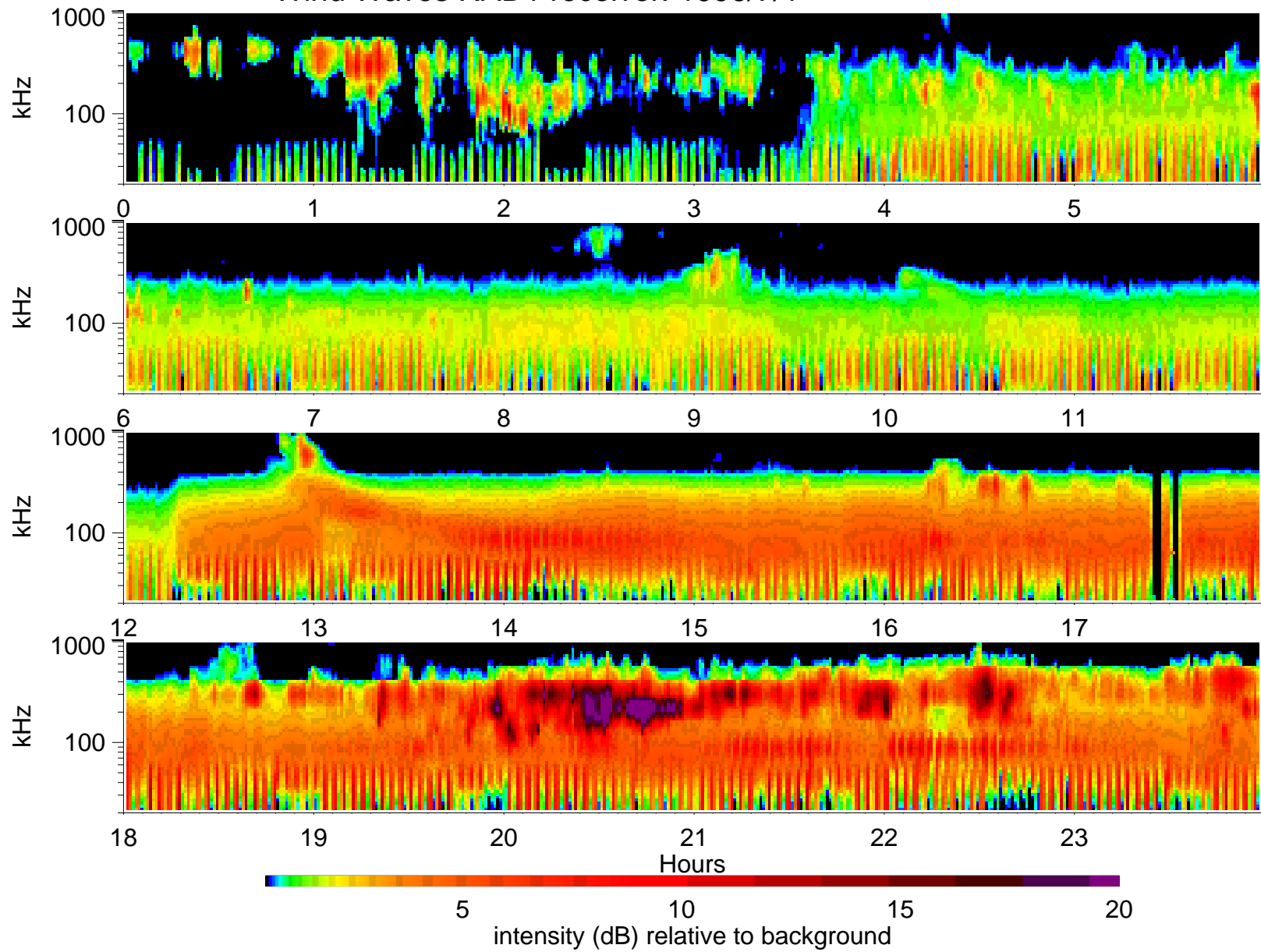
Wind Waves RAD1 receiver: 1996/7/1
