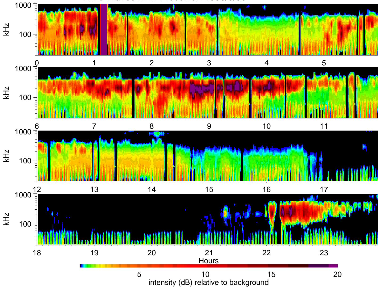
Wind Waves RAD1 receiver: 1996/6/30
