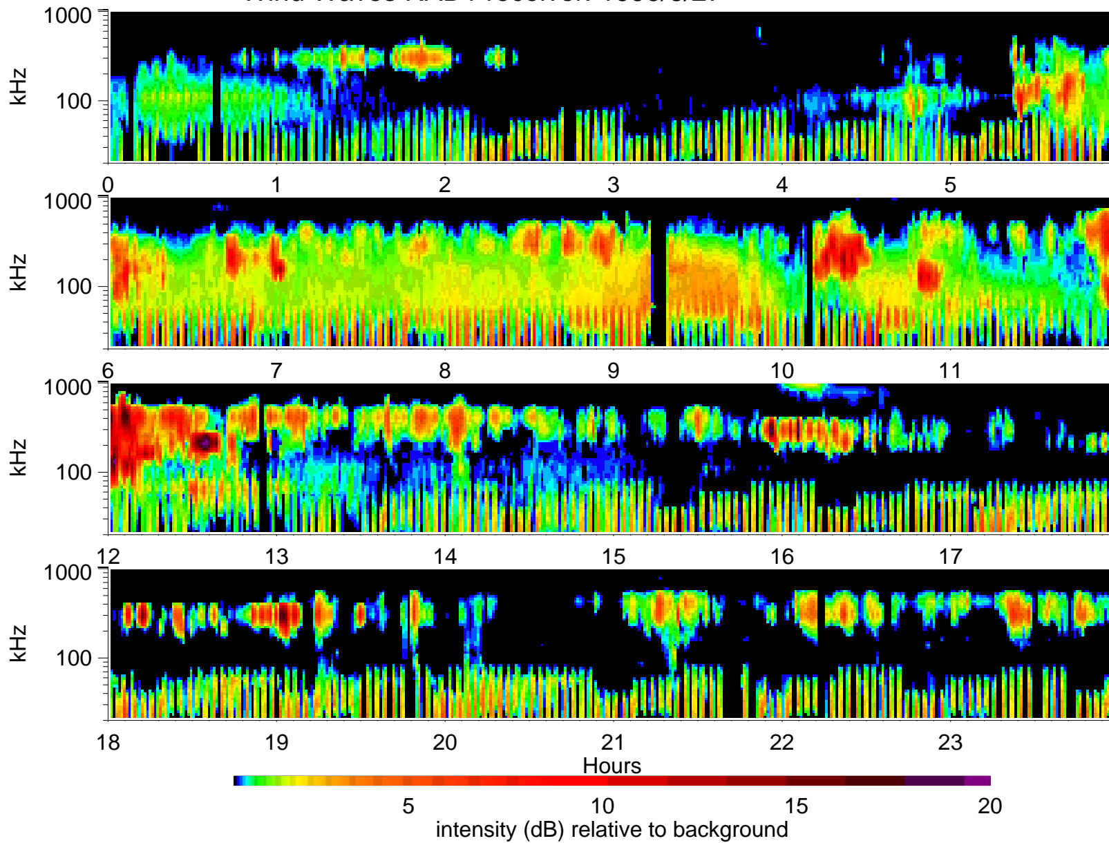
Wind Waves RAD1 receiver: 1996/6/27
