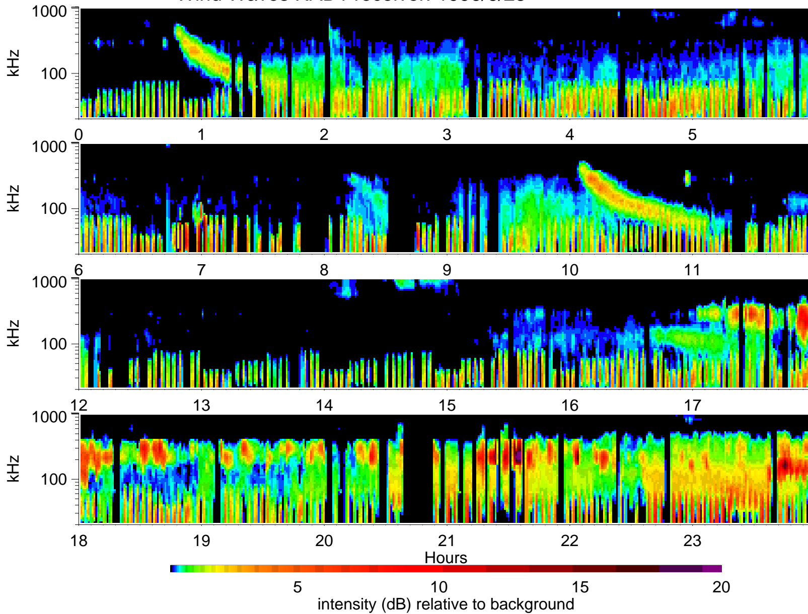
Wind Waves RAD1 receiver: 1996/6/25
