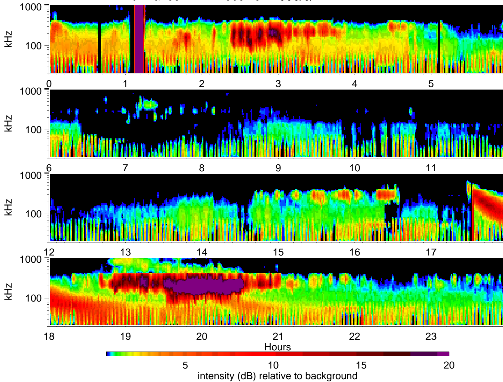
Wind Waves RAD1 receiver: 1996/6/24
