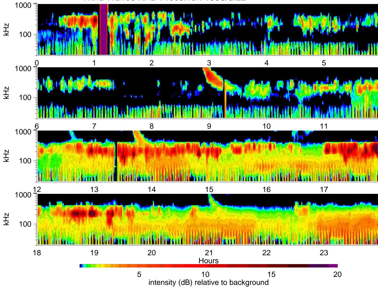
Wind Waves RAD1 receiver: 1996/6/22
