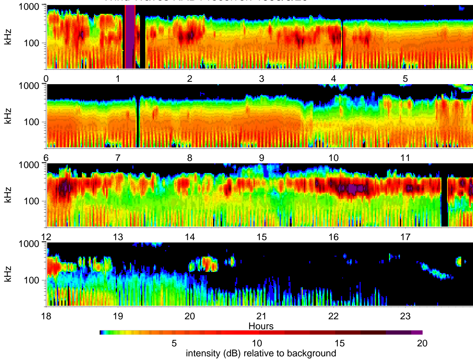
Wind Waves RAD1 receiver: 1996/6/20
