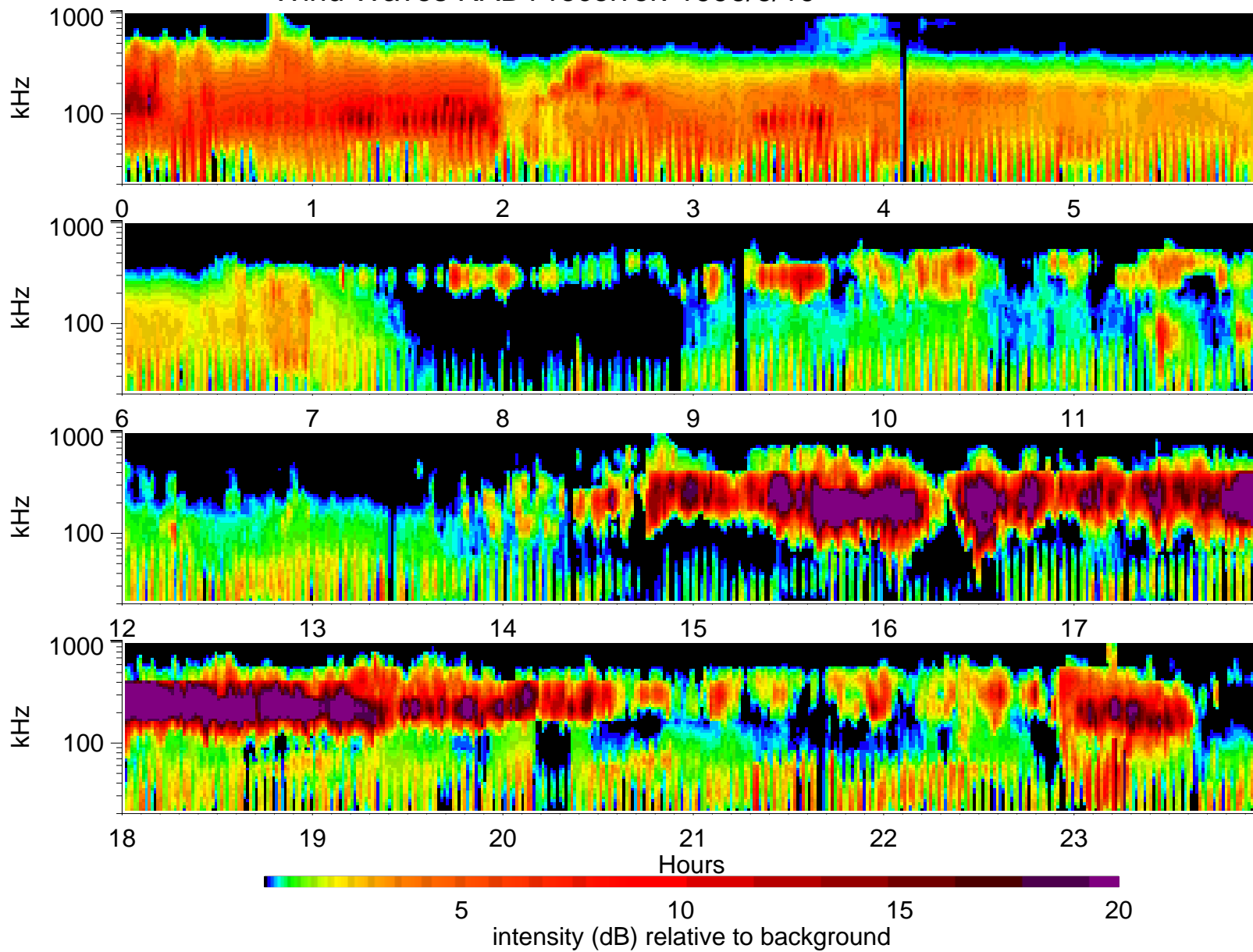
Wind Waves RAD1 receiver: 1996/6/19
