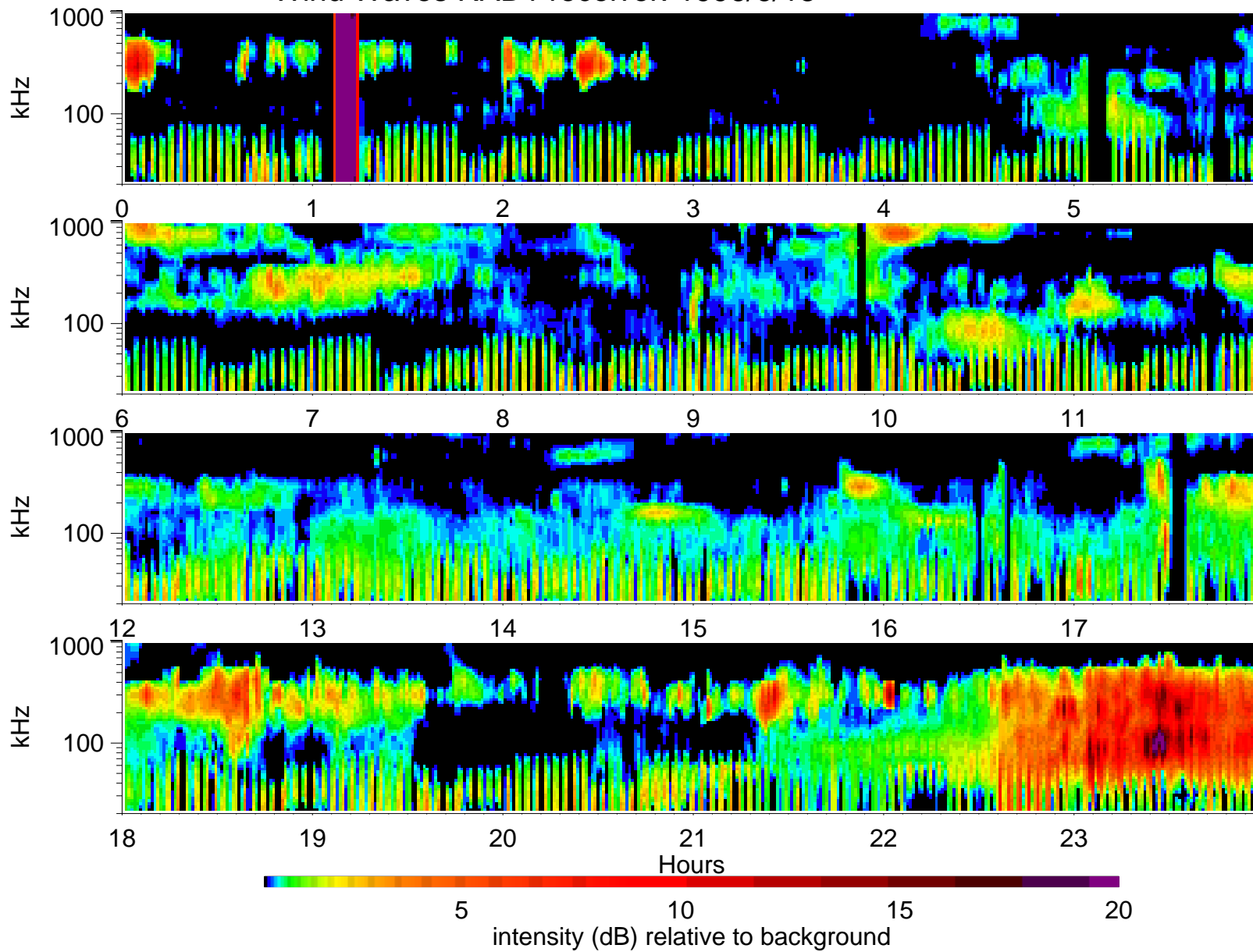
Wind Waves RAD1 receiver: 1996/6/18
