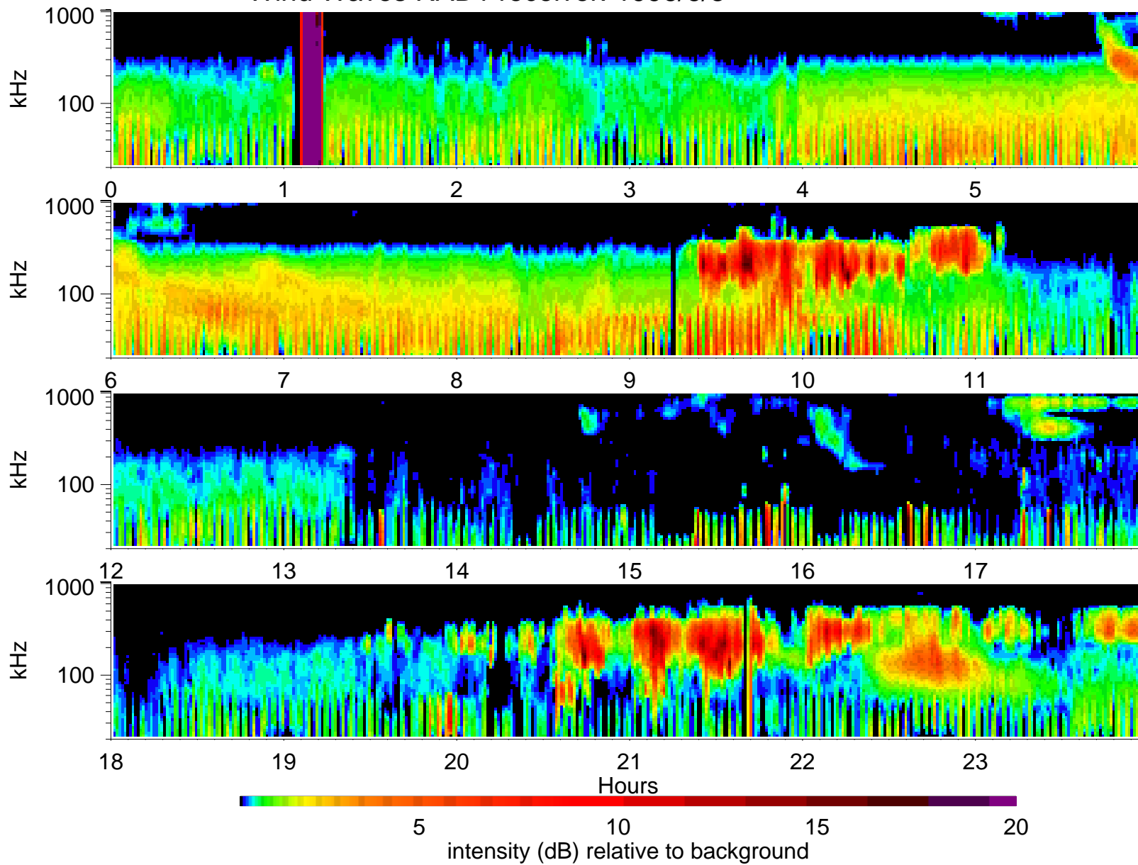
Wind Waves RAD1 receiver: 1996/6/8
