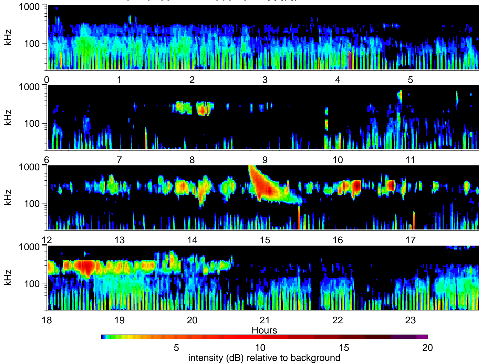
Wind Waves RAD1 receiver: 1996/6/7
