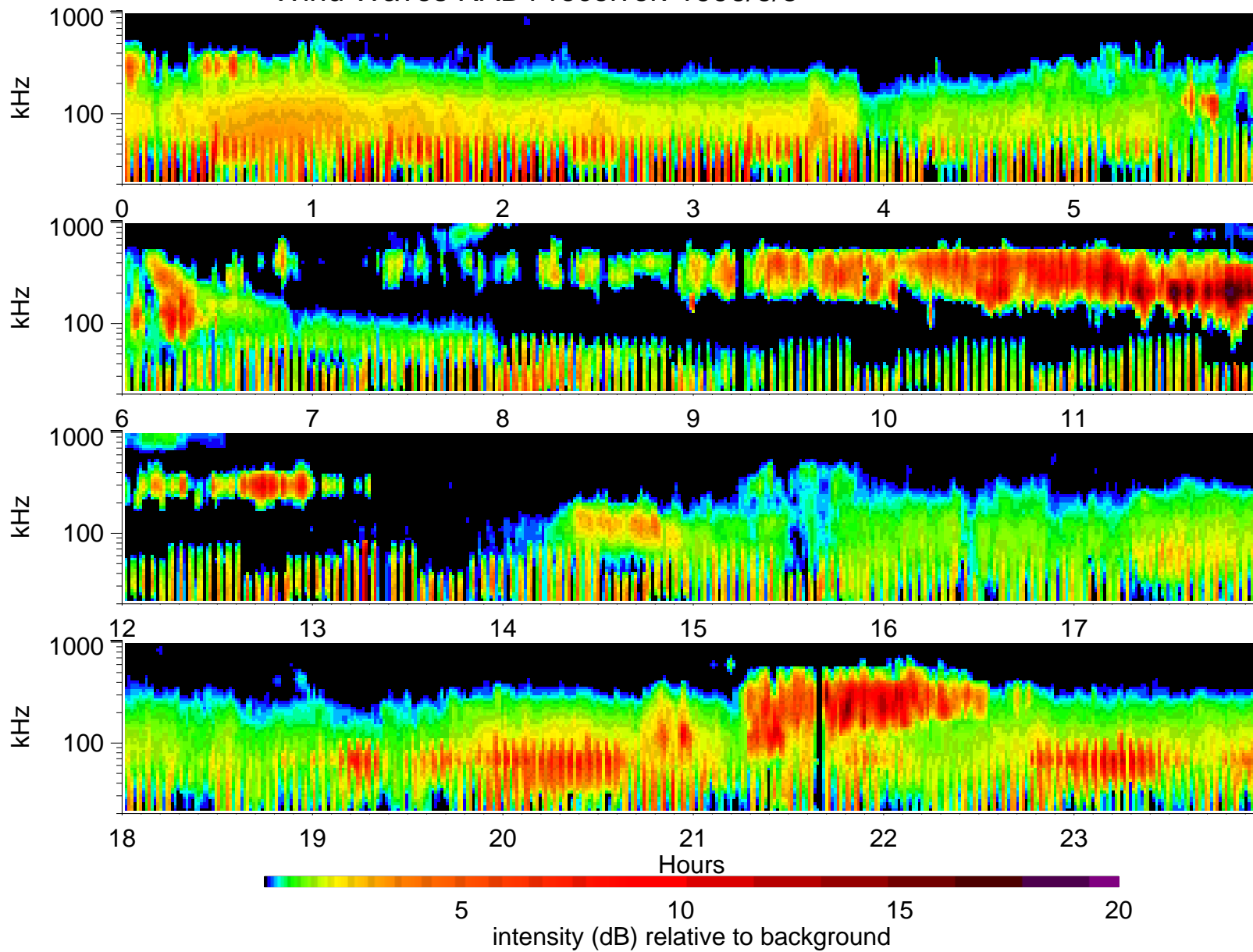
Wind Waves RAD1 receiver: 1996/6/5
