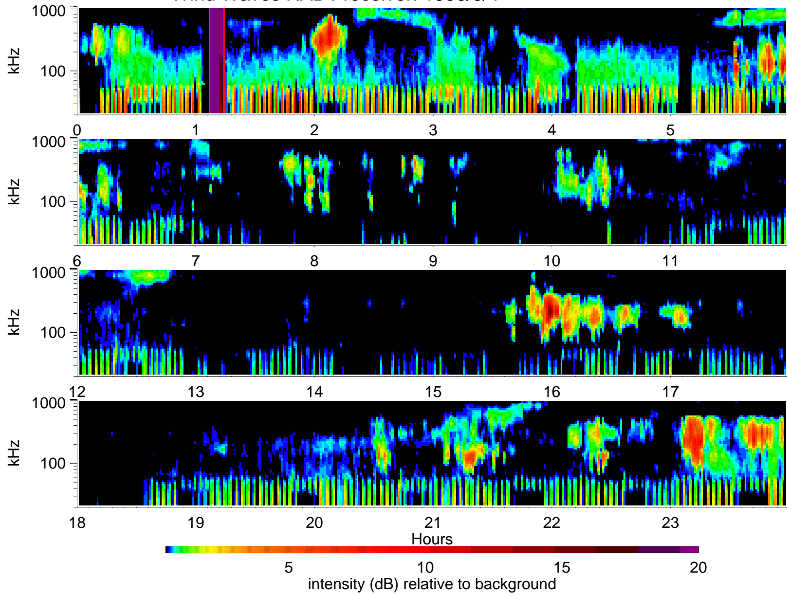
Wind Waves RAD1 receiver: 1996/6/4
