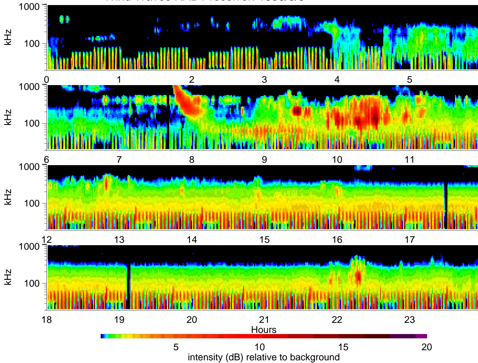
Wind Waves RAD1 receiver: 1996/6/3
