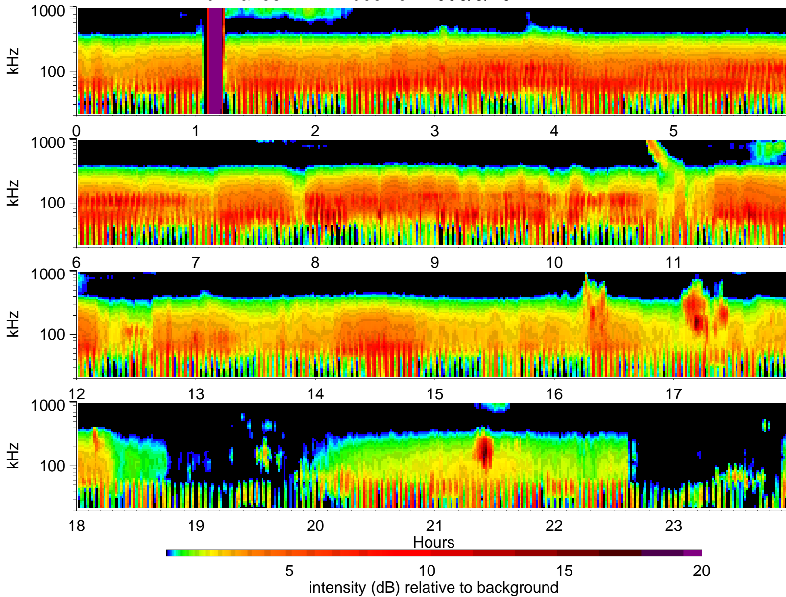
Wind Waves RAD1 receiver: 1996/5/29
