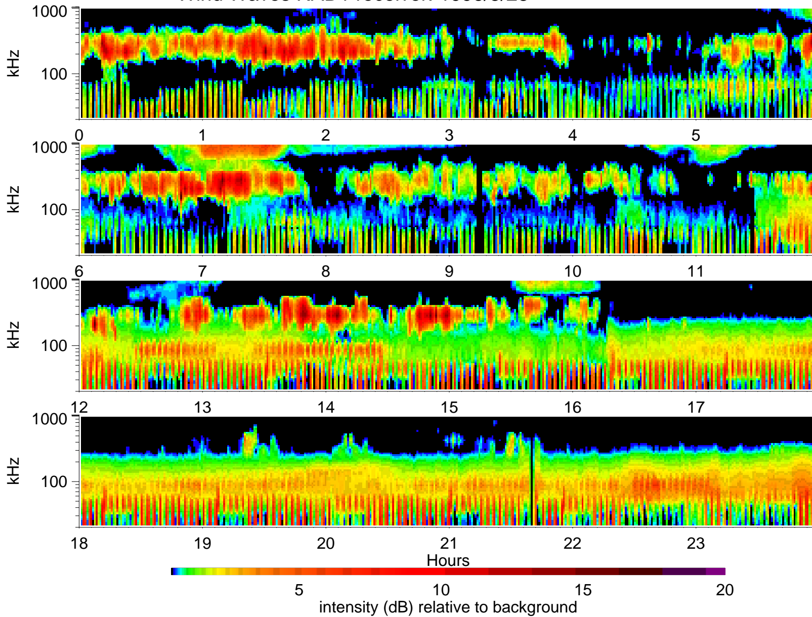
Wind Waves RAD1 receiver: 1996/5/28
