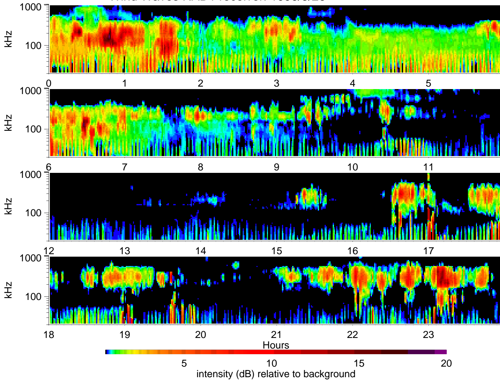
Wind Waves RAD1 receiver: 1996/5/26
