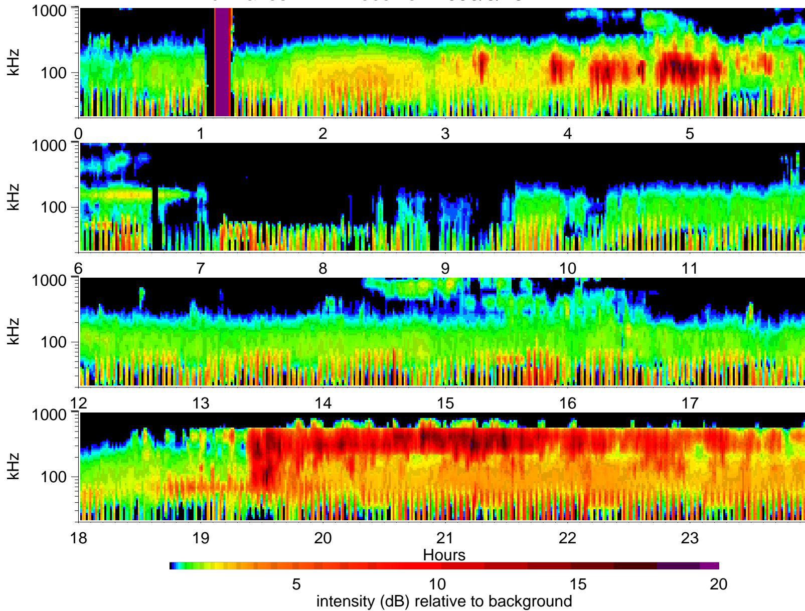
Wind Waves RAD1 receiver: 1996/5/25
