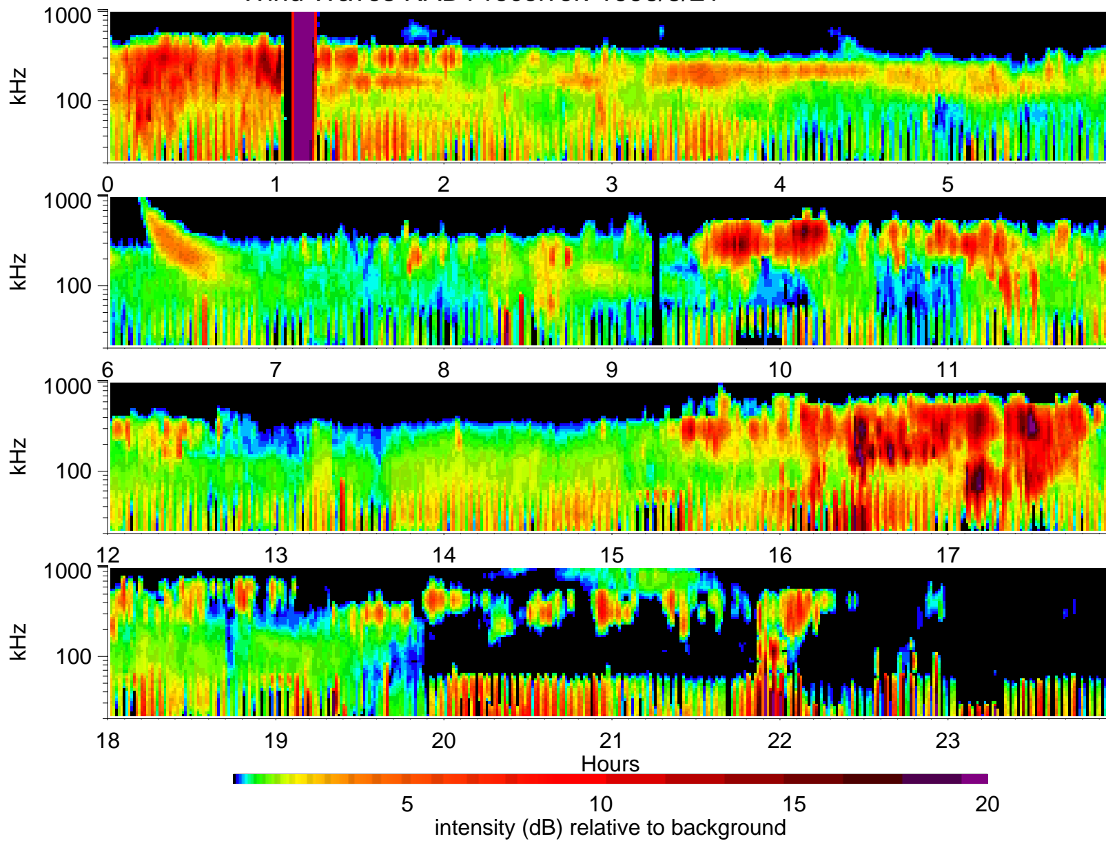
Wind Waves RAD1 receiver: 1996/5/21
