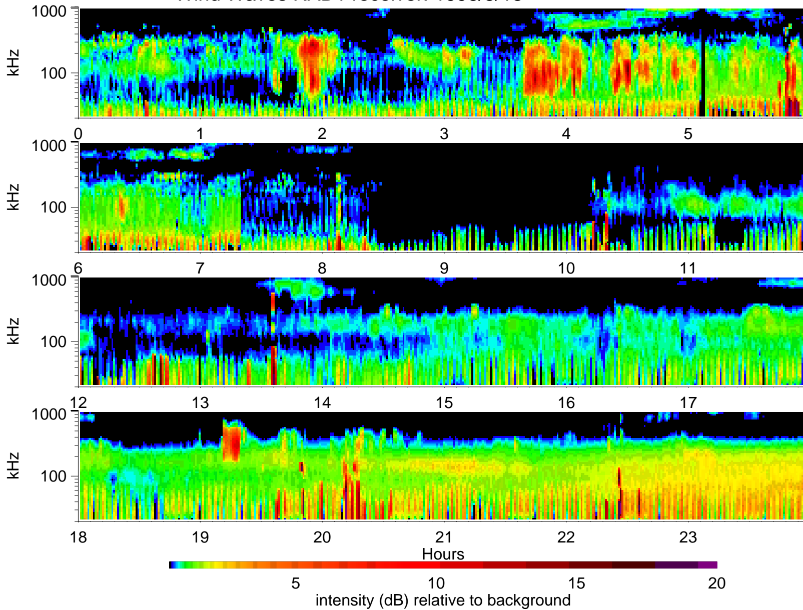
Wind Waves RAD1 receiver: 1996/5/18
