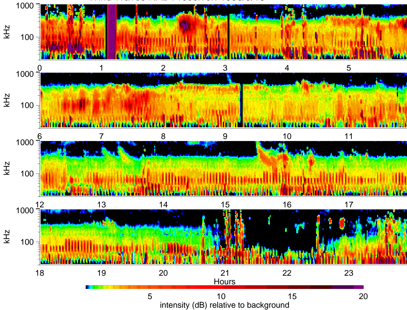
Wind Waves RAD1 receiver: 1996/5/13
