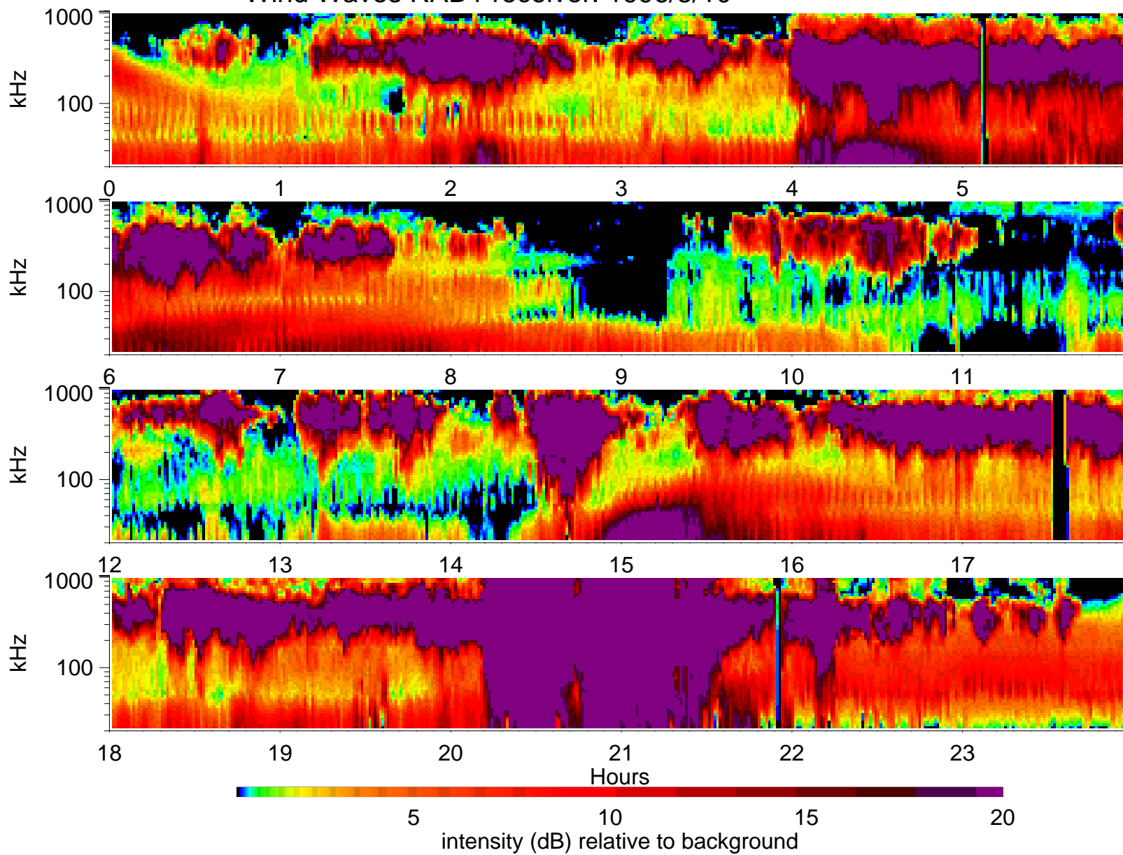
Wind Waves RAD1 receiver: 1996/5/10
