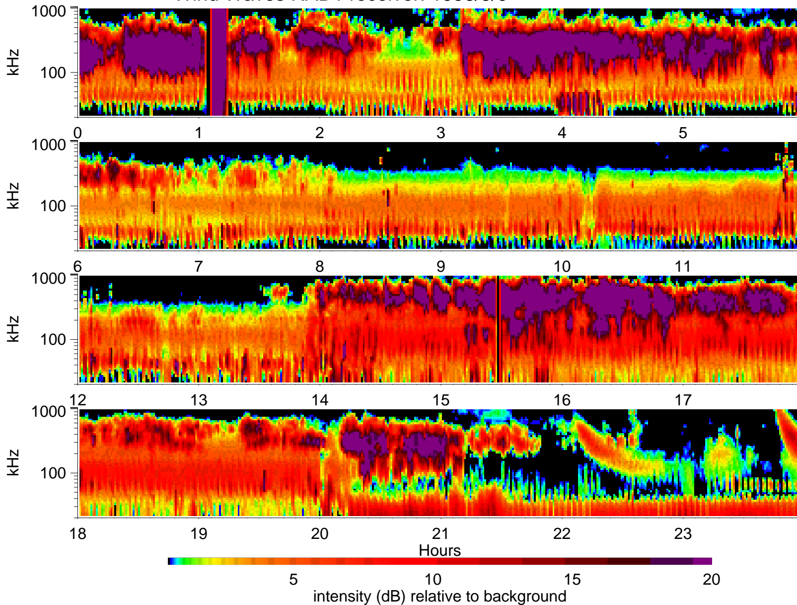
Wind Waves RAD1 receiver: 1996/5/9
