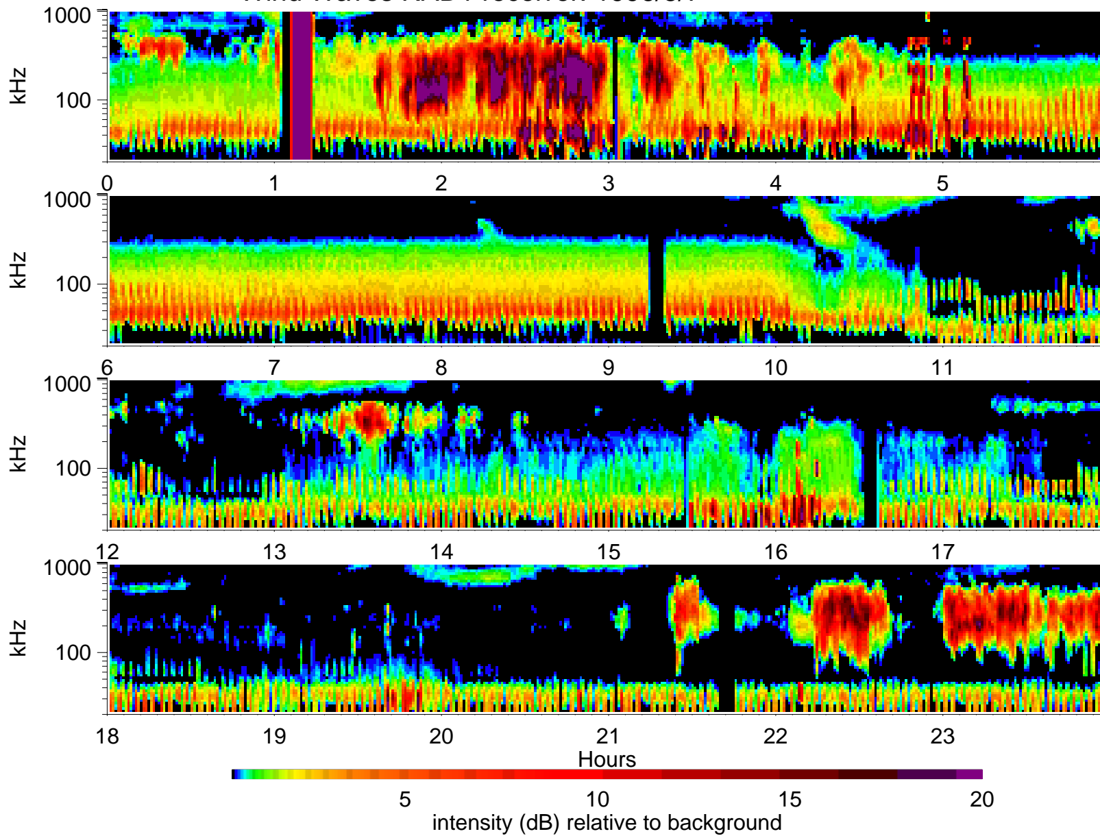
Wind Waves RAD1 receiver: 1996/5/7
