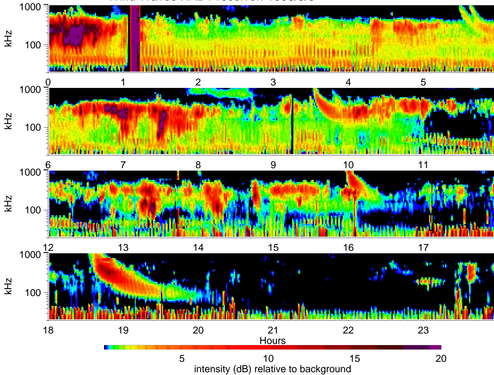
Wind Waves RAD1 receiver: 1996/5/5
