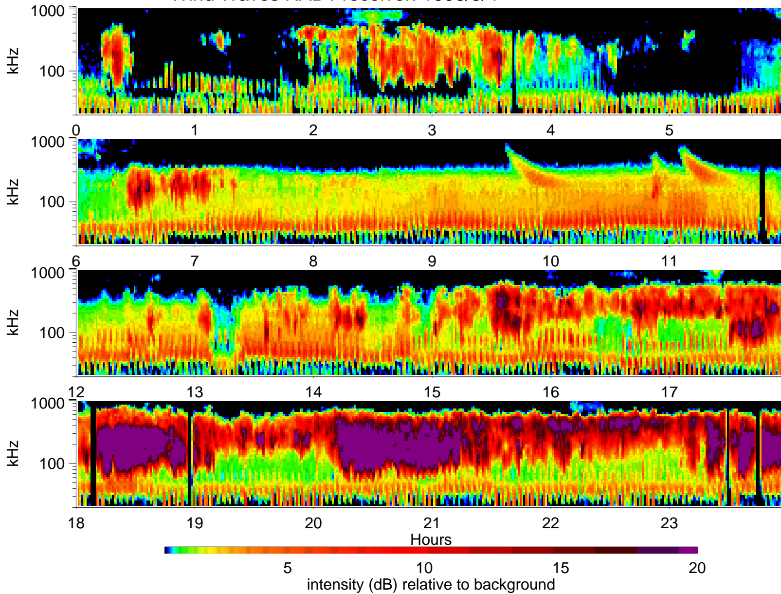
Wind Waves RAD1 receiver: 1996/5/4
