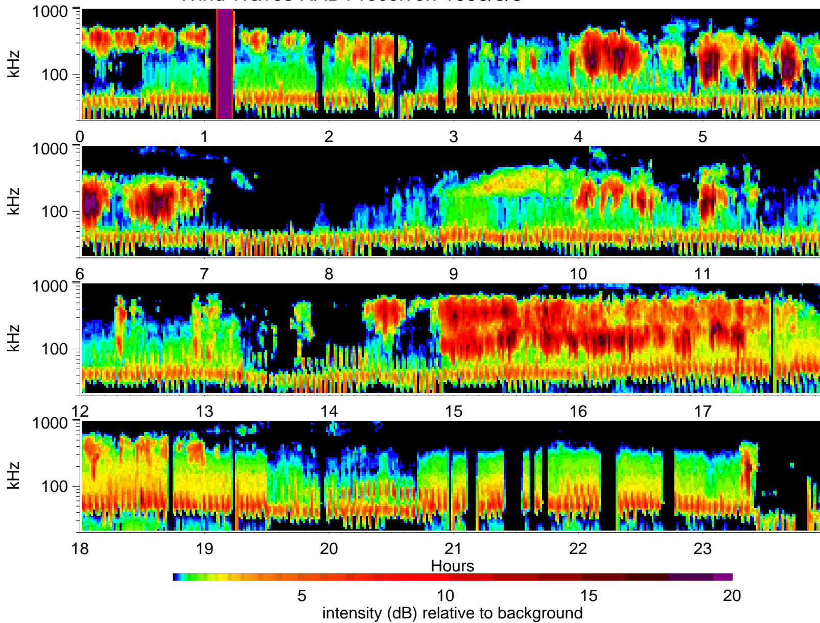
Wind Waves RAD1 receiver: 1996/5/3
