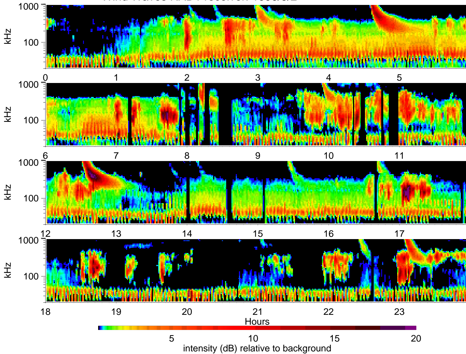
Wind Waves RAD1 receiver: 1996/5/2
