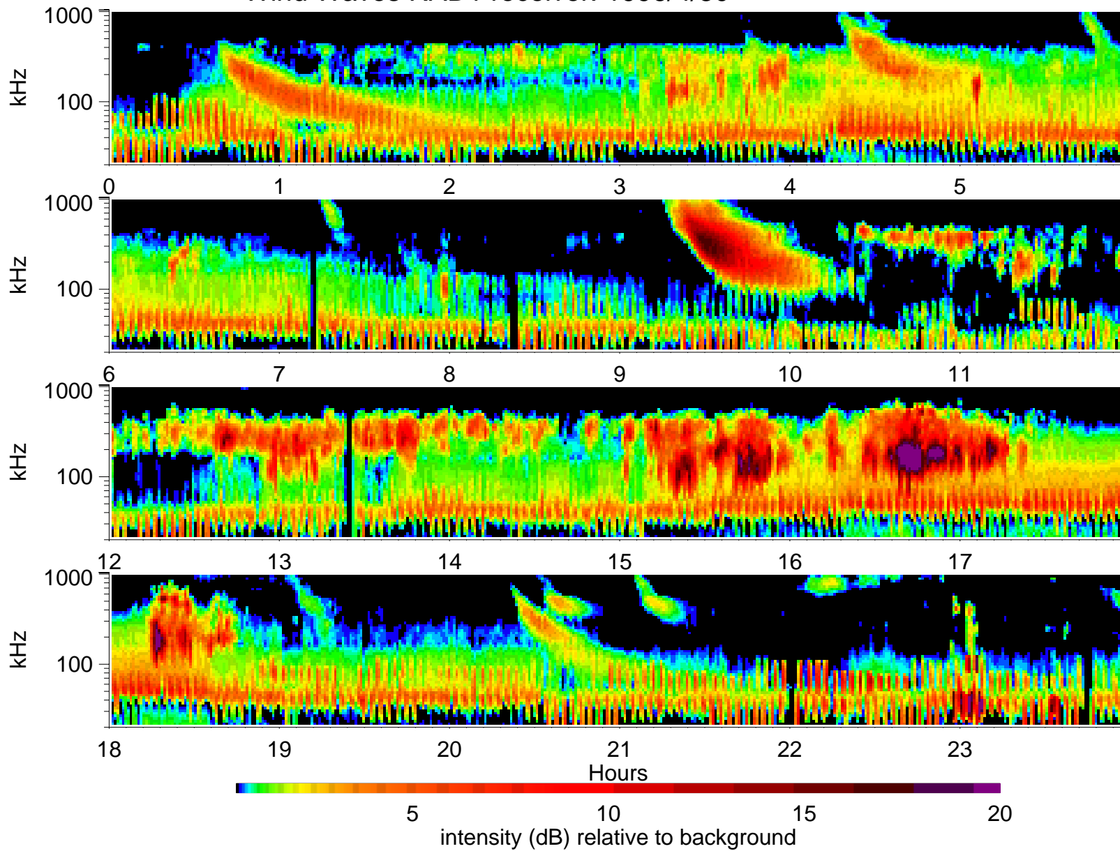
Wind Waves RAD1 receiver: 1996/4/30
