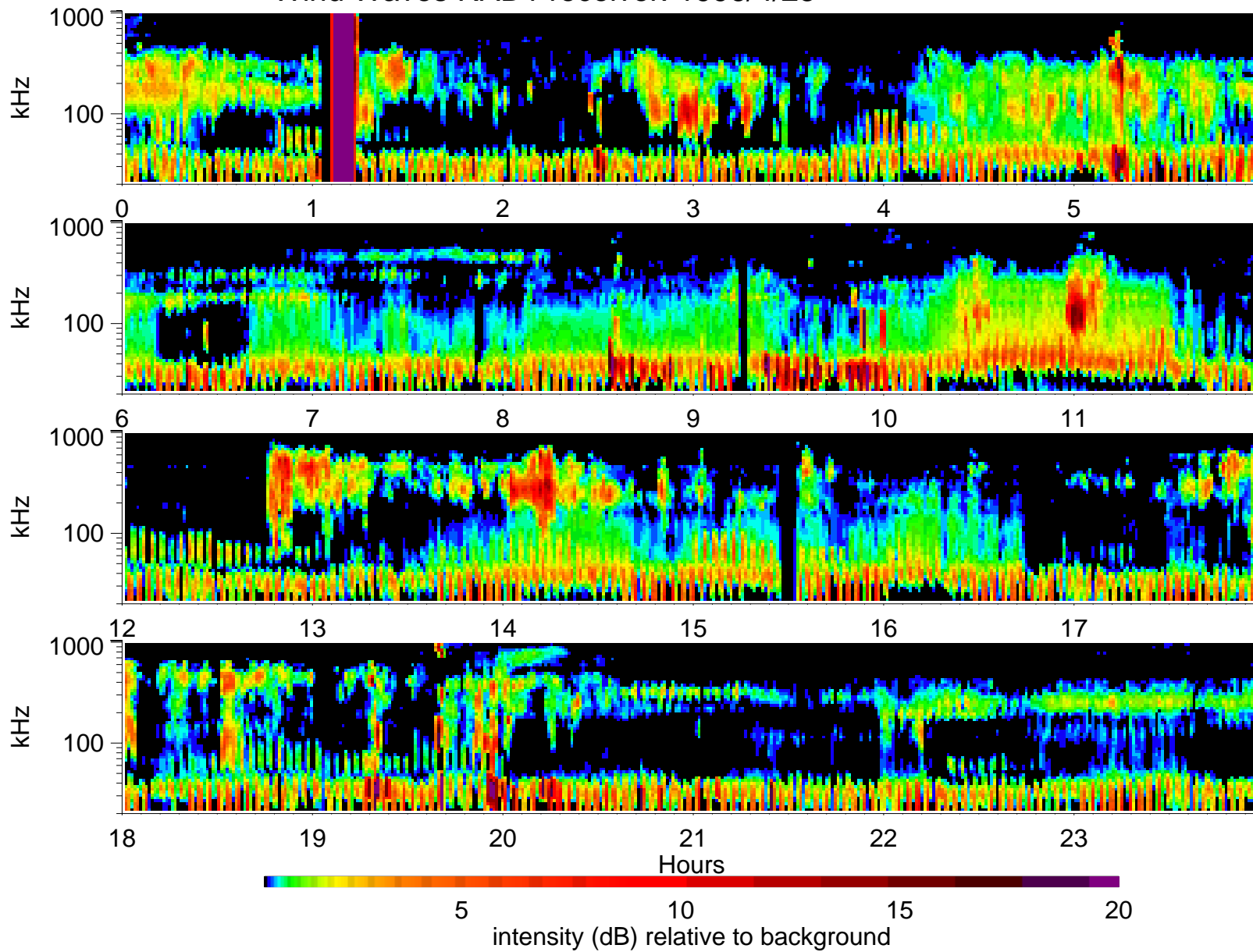
Wind Waves RAD1 receiver: 1996/4/25
