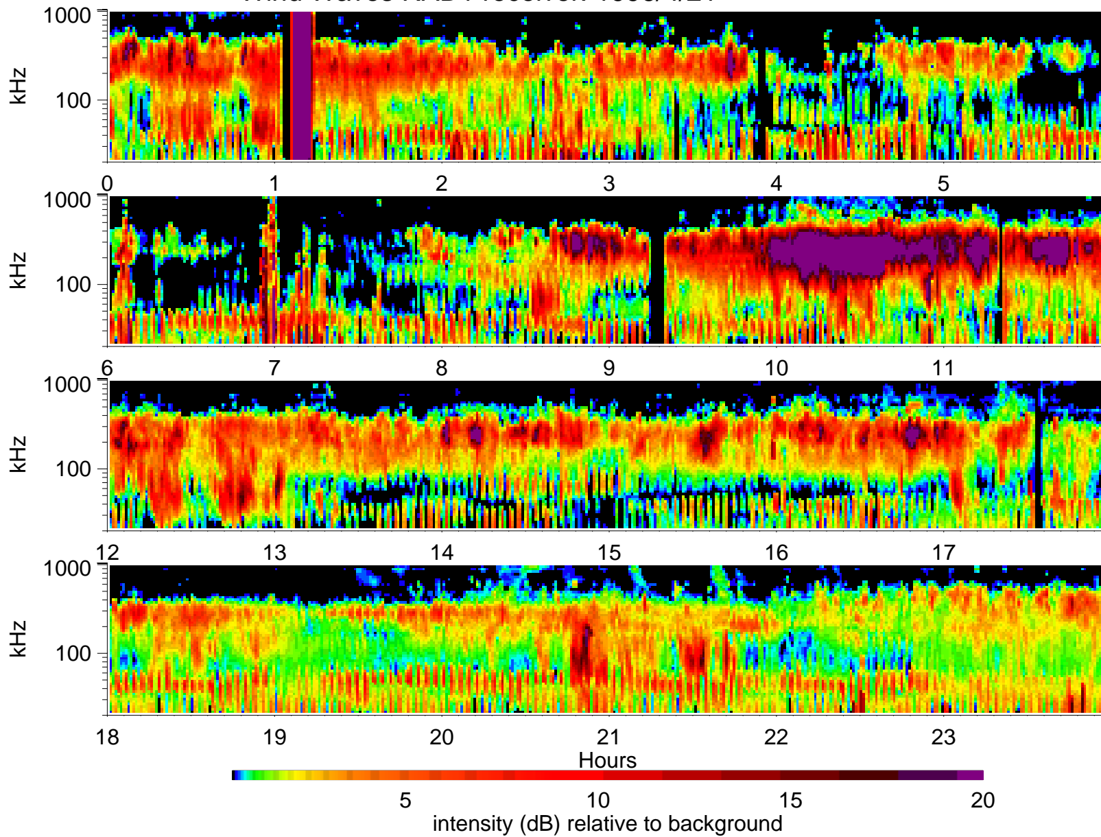
Wind Waves RAD1 receiver: 1996/4/21
