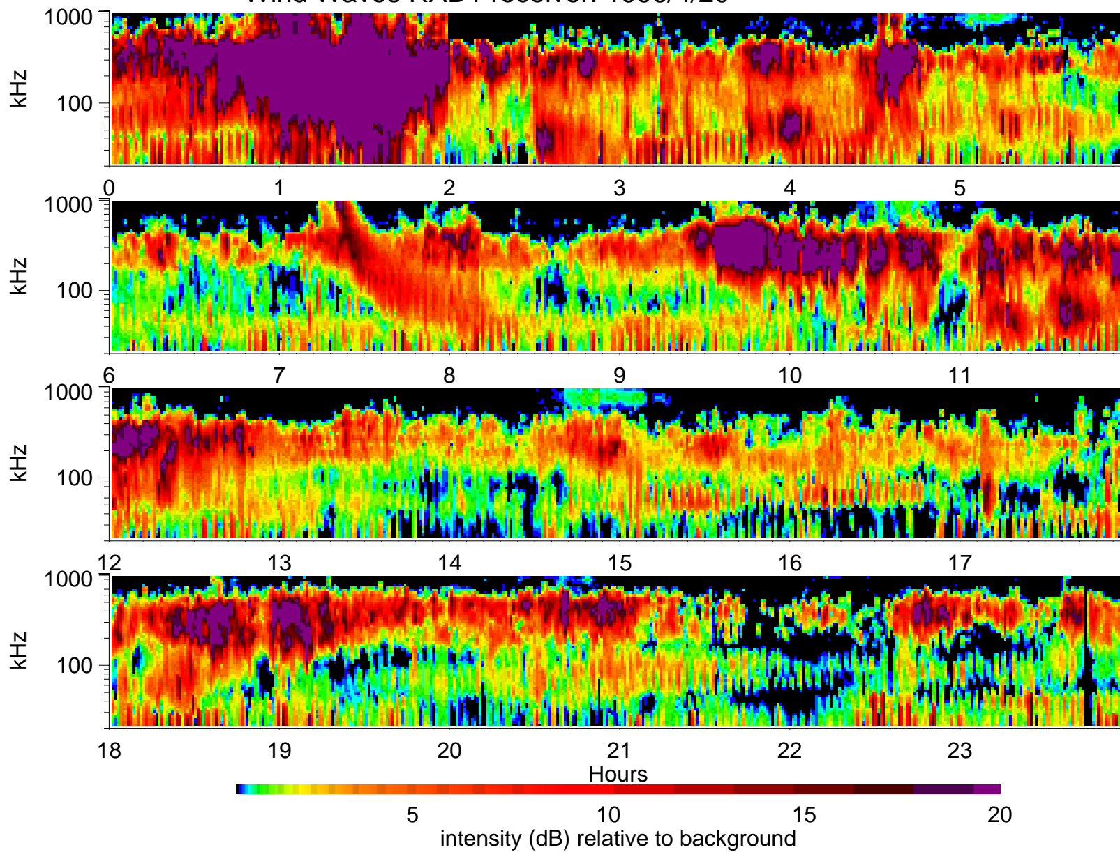
Wind Waves RAD1 receiver: 1996/4/20
