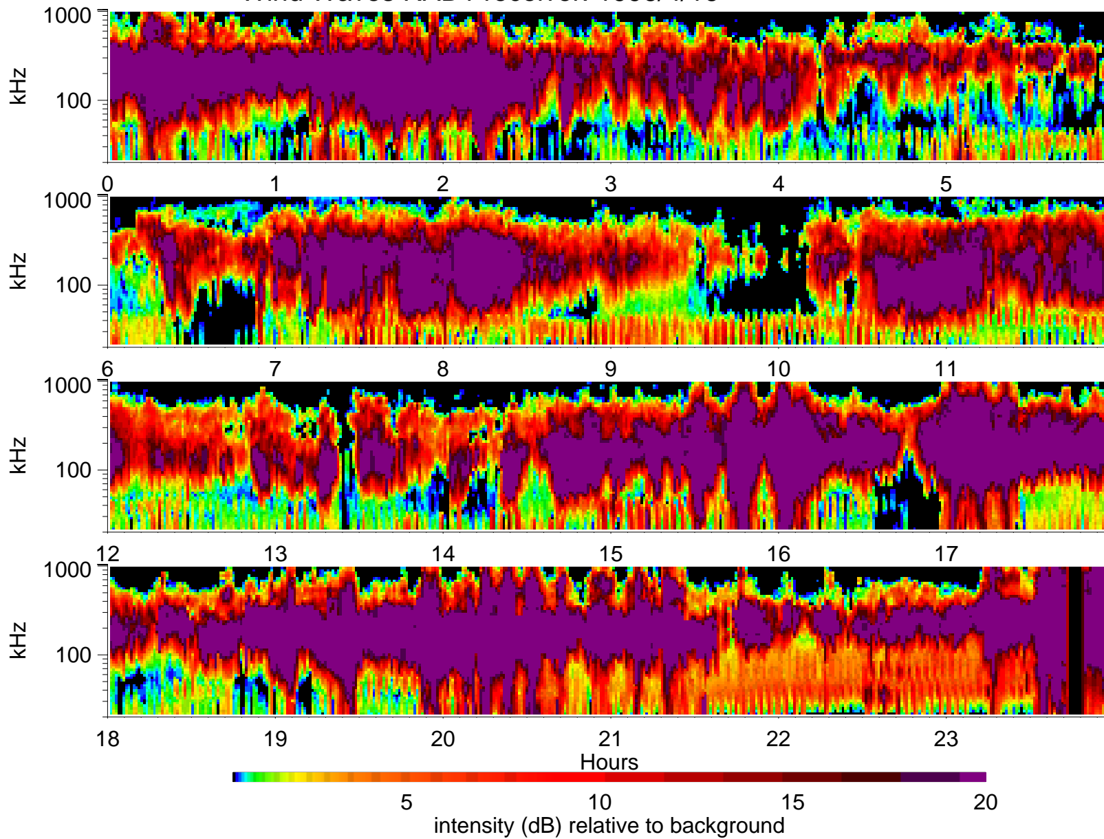
Wind Waves RAD1 receiver: 1996/4/16
