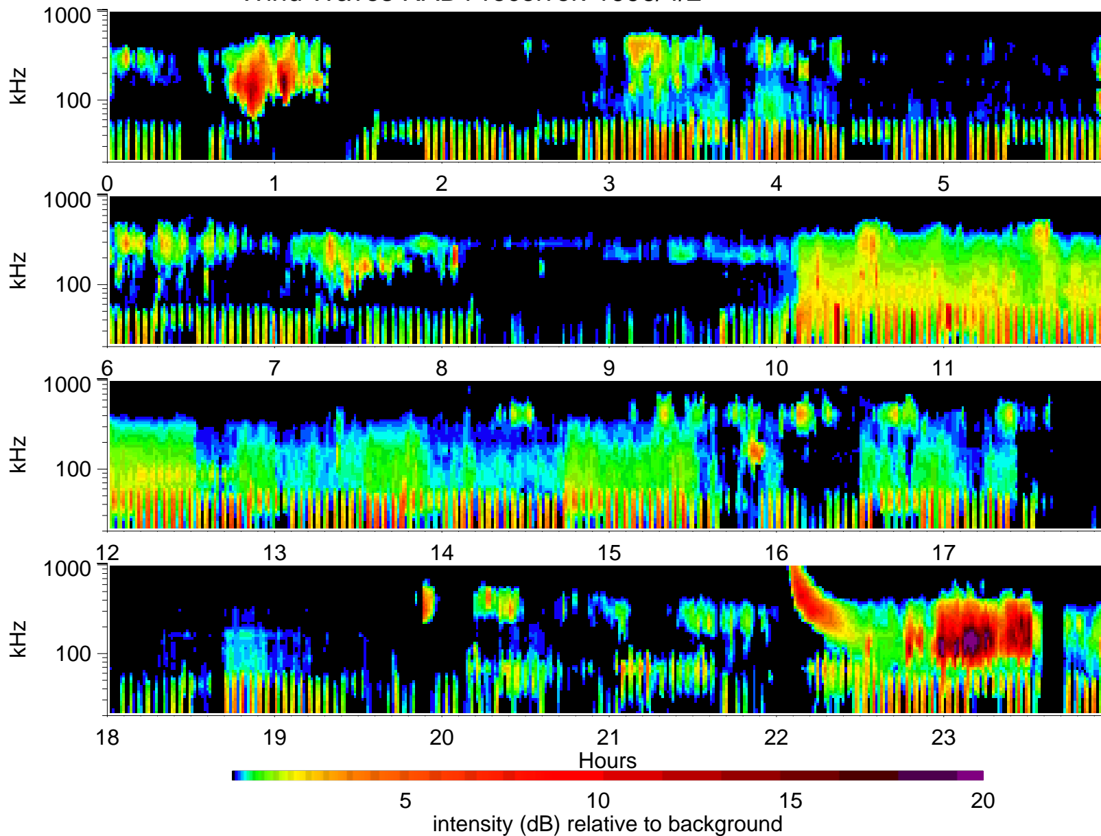
Wind Waves RAD1 receiver: 1996/4/2
