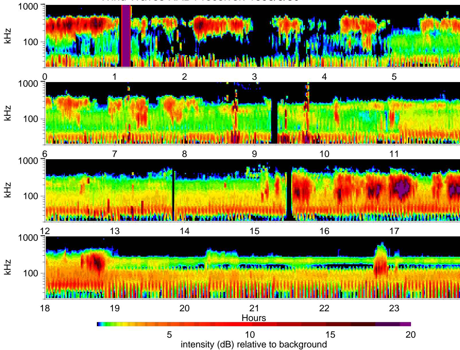
Wind Waves RAD1 receiver: 1996/3/30
