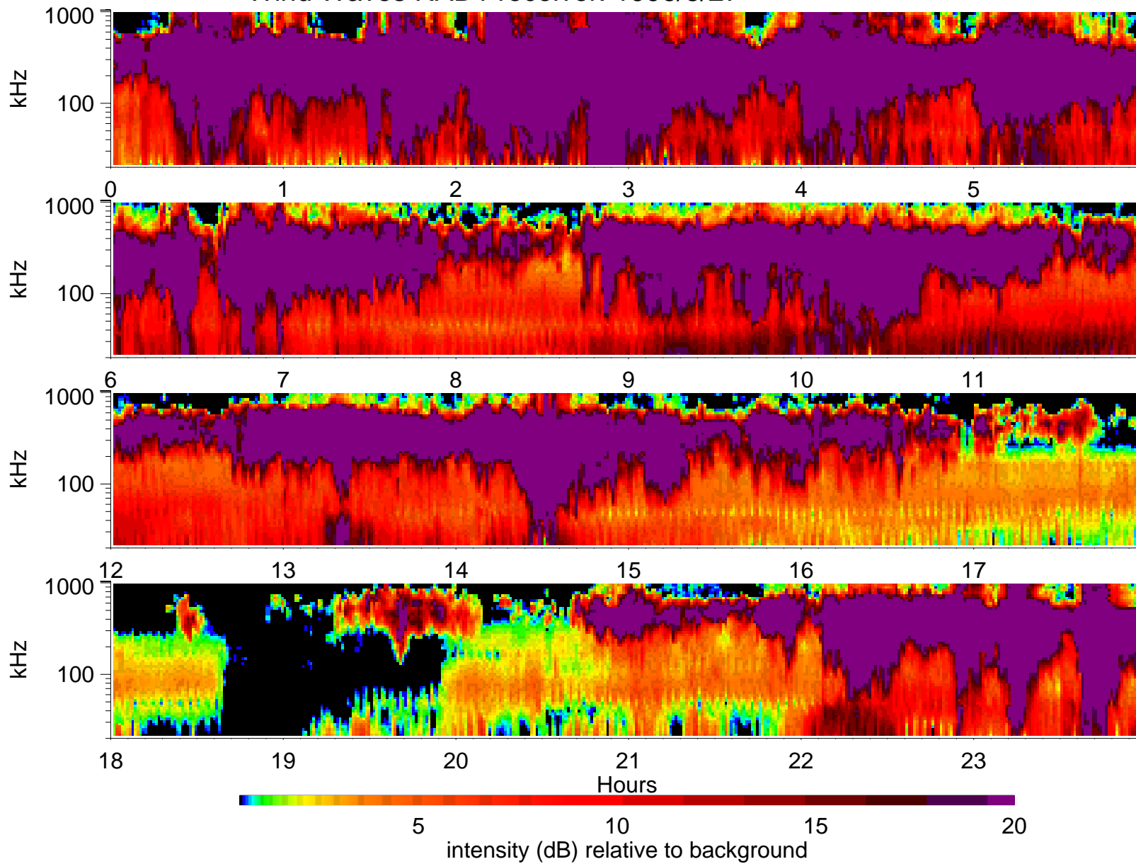
Wind Waves RAD1 receiver: 1996/3/27
