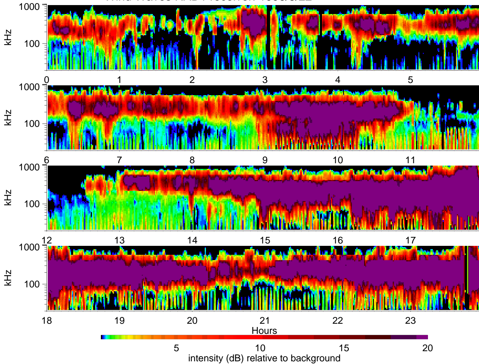
Wind Waves RAD1 receiver: 1996/3/22
