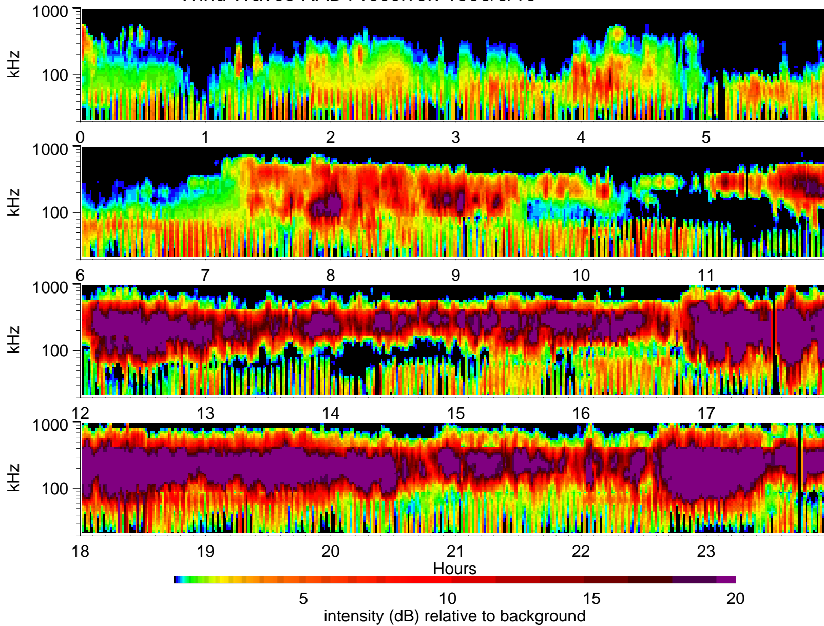
Wind Waves RAD1 receiver: 1996/3/19
