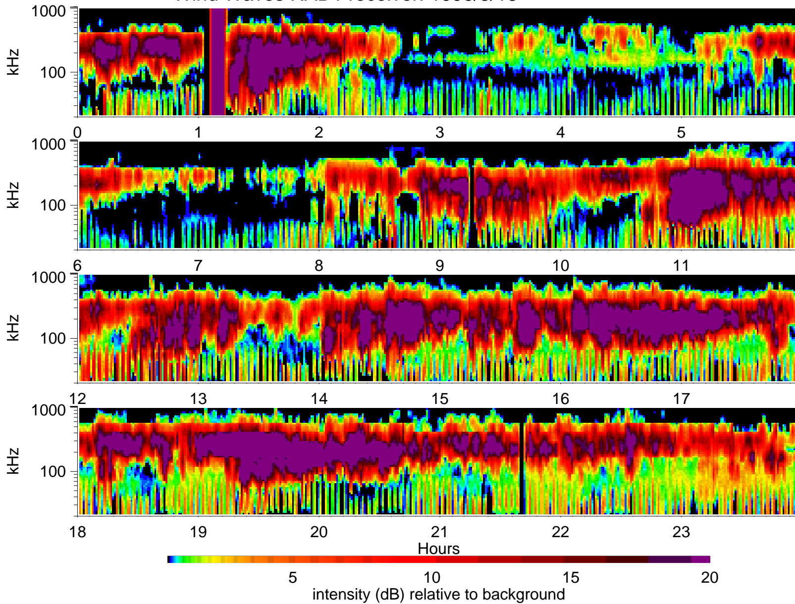
Wind Waves RAD1 receiver: 1996/3/18
