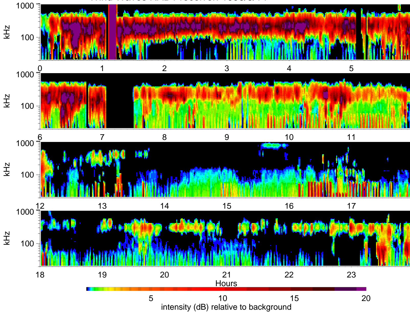
Wind Waves RAD1 receiver: 1996/3/14
