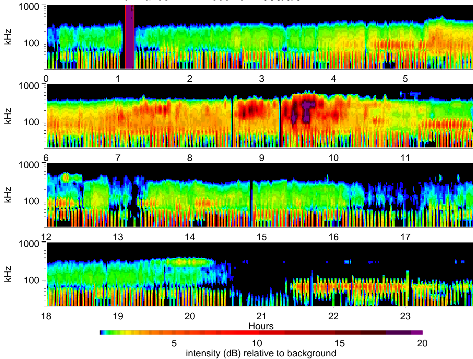
Wind Waves RAD1 receiver: 1996/3/8
