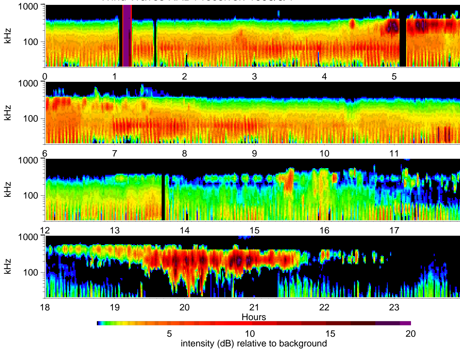
Wind Waves RAD1 receiver: 1996/3/4
