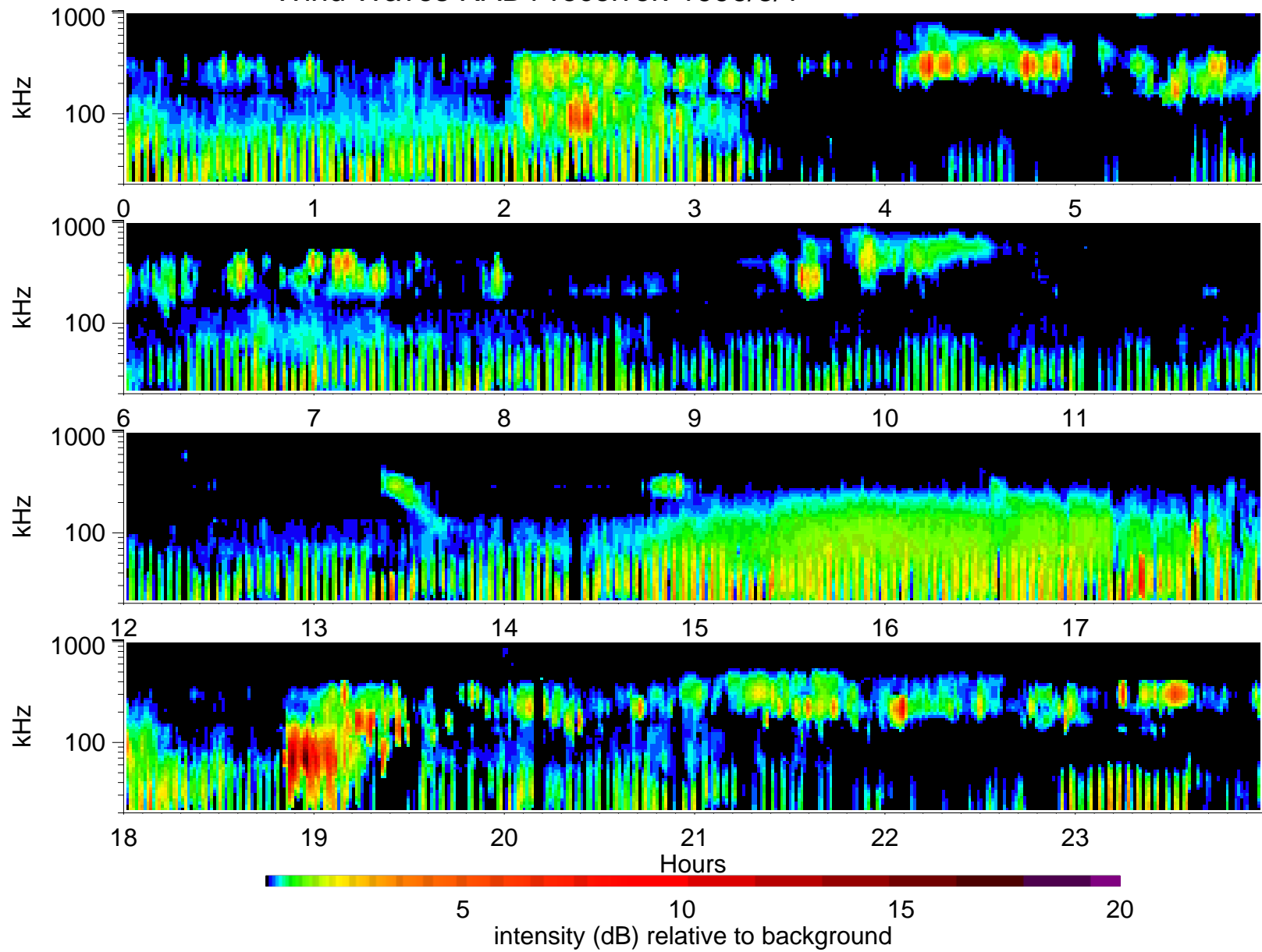
Wind Waves RAD1 receiver: 1996/3/1
