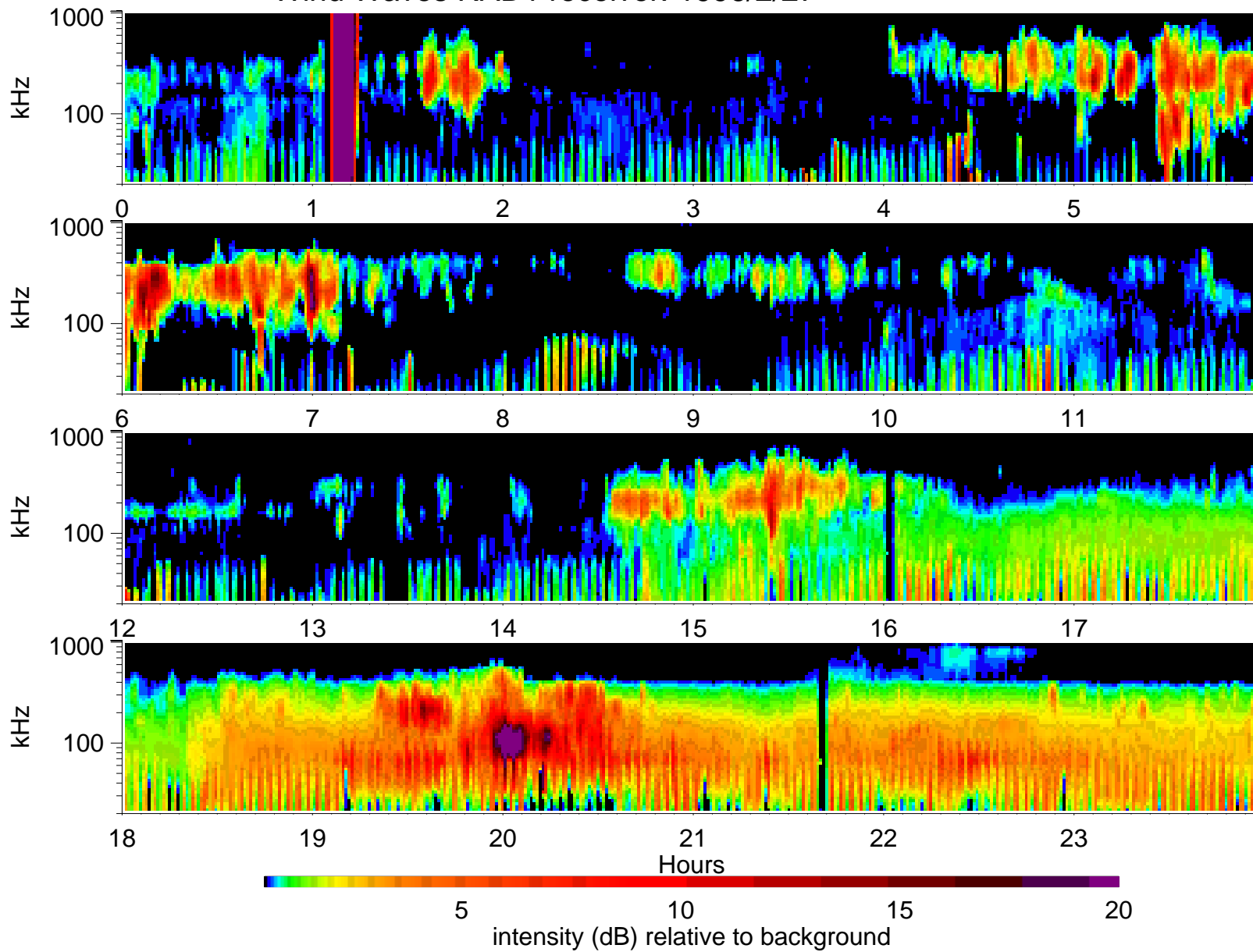
Wind Waves RAD1 receiver: 1996/2/27
