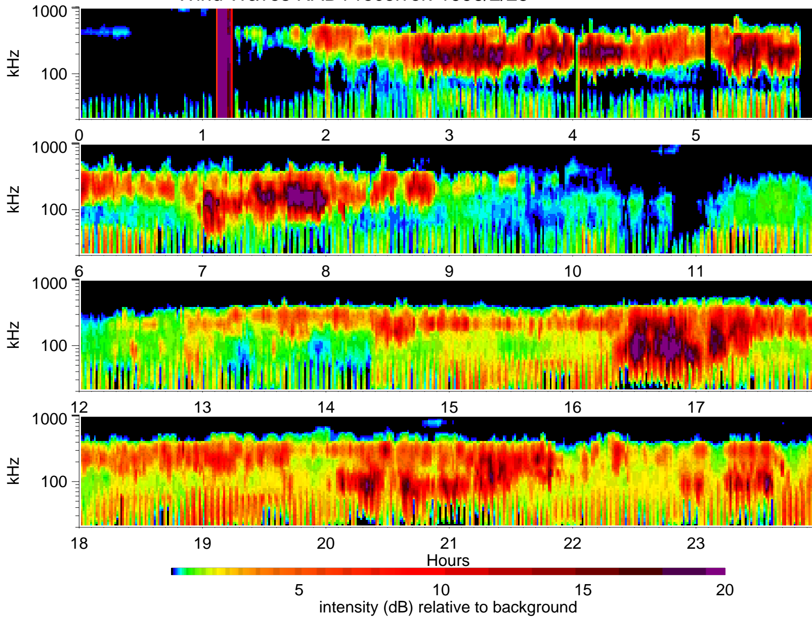
Wind Waves RAD1 receiver: 1996/2/25
