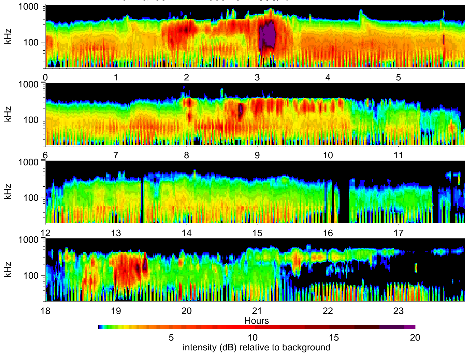
Wind Waves RAD1 receiver: 1996/2/24
